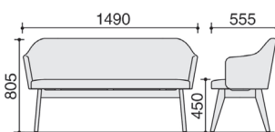
K04-(D·Z)058S
