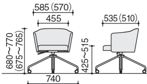
K04-(W·B·M)G18·G28
