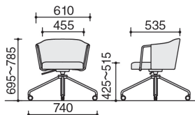
K04-(W·B·M)G21
