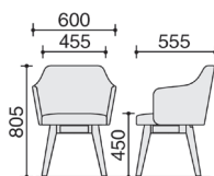
K04-(D·Z)038S
